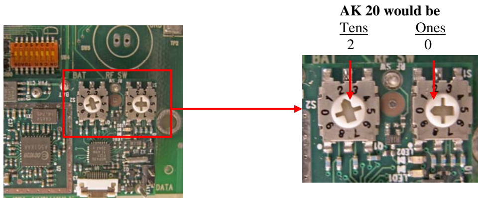
Figure 3-2. SLTX Synthesizer Board
