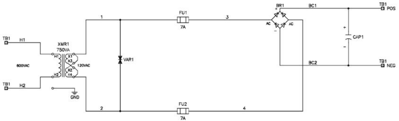
Figure 2: Brake Rectifier Schematic (Single Brake Coil)
