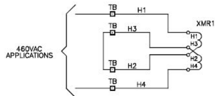
Figure 3: Brake Rectifier Schematic (Dual Brake Coil)
