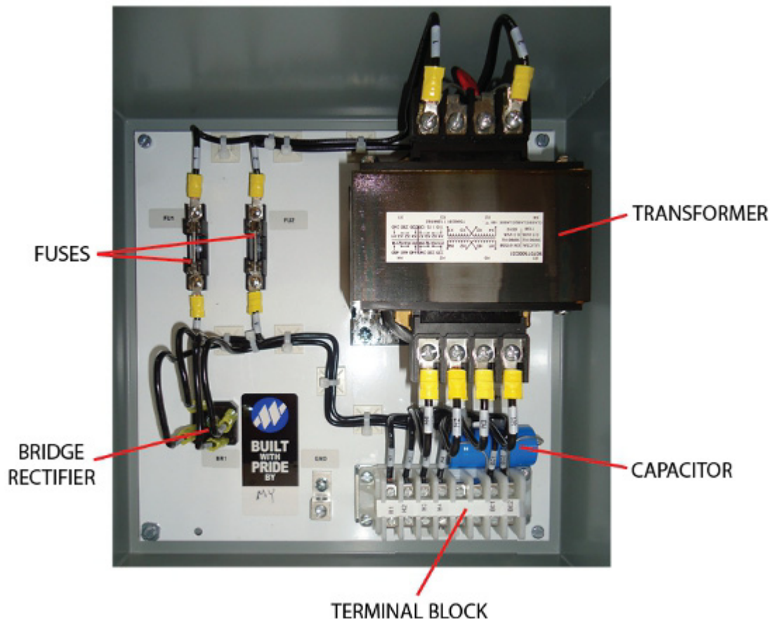
Figure 1: Brake Rectifier
